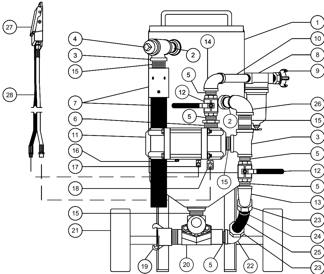
1" Piping with Combo-Micro Valve
